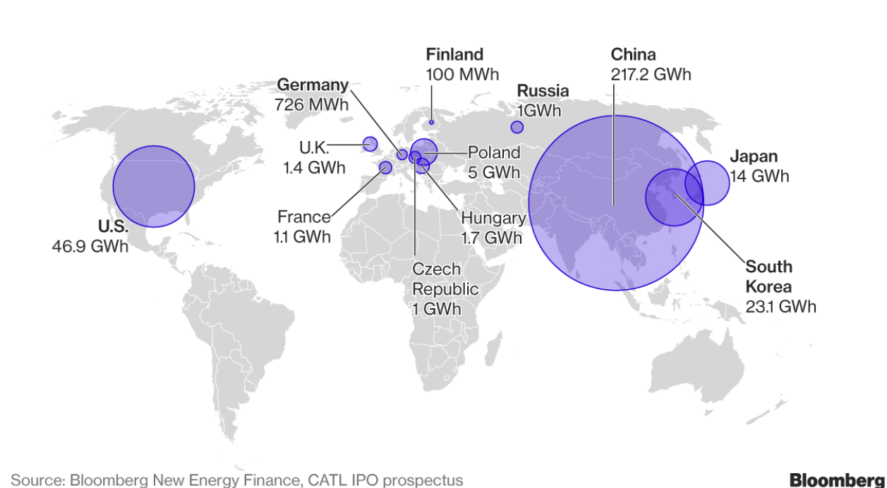
Figure 1-3: Planned and Existing Battery Cell Production Capacity
