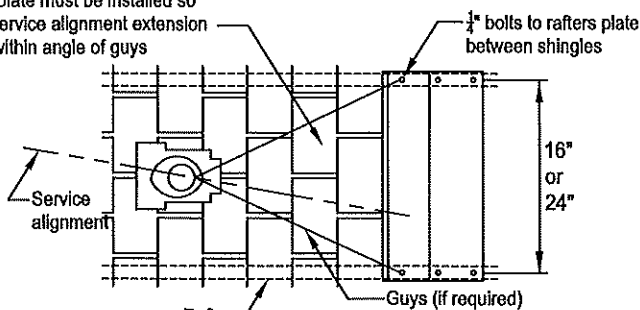
GUY DETAIL
