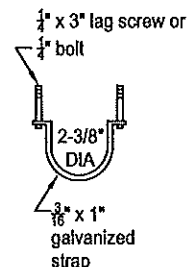
ANCHOR STRAP No. 1 (OR EQUAL)
