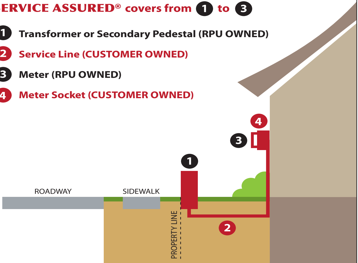
FIGURE 2 Underground Electric Service
